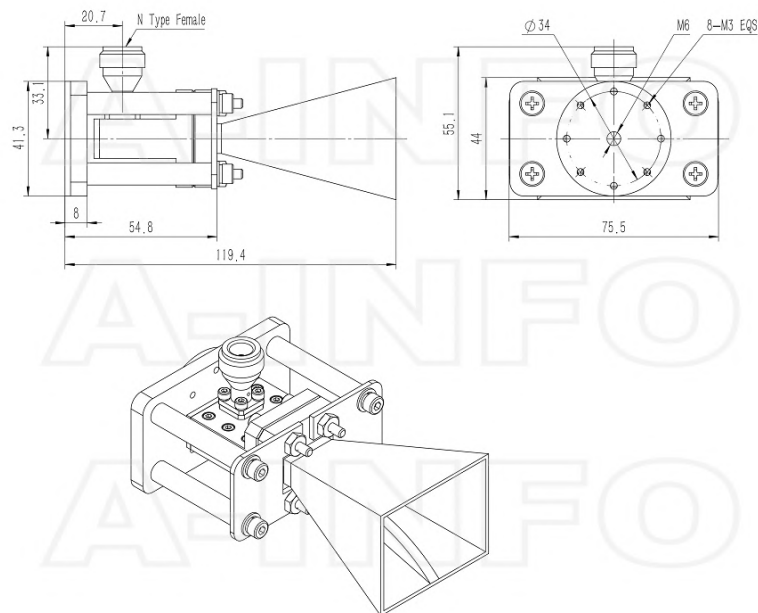
N-Female Output with Round Mounting Bracket (Option, P/N: LB-65180-10-C-MB)
