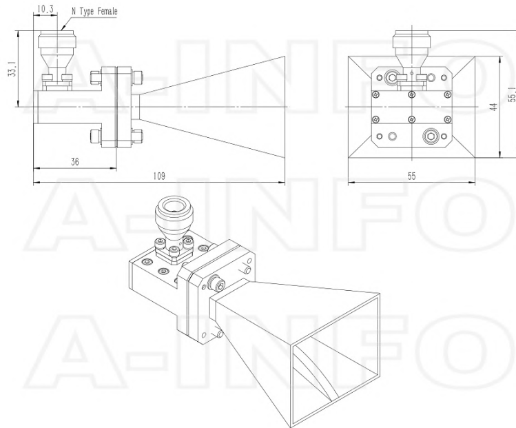
N-Female Output (P/N: LB-60180-NF)
