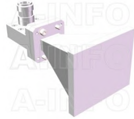
LB-60180-HNFSPS Broadband Horn Antenna 6-18GHz 10dB Gain High Power N Type Female
