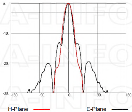
Frequency: 22.0GHz
