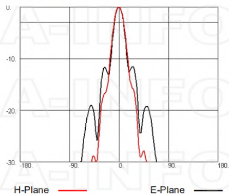
Frequency: 26.0GHz
