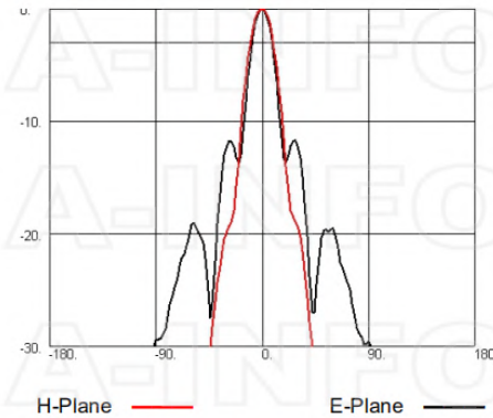
Frequency: 24.0GHz
