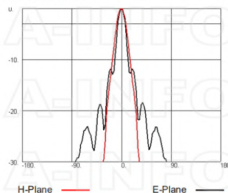
Frequency: 32.0GHz
