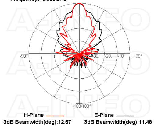
Frequency:16.000GHz
