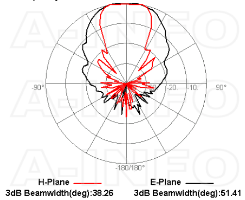
Frequency:12.000GHz
