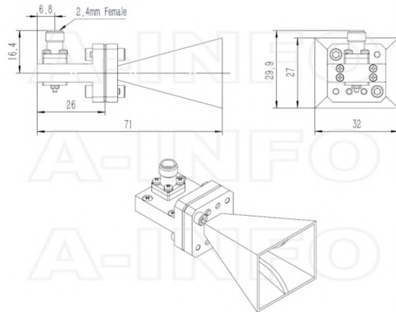
2.4mm-Female Output with Round Mounting Bracket (Option, P/N: LB-180400-10-C-MB)
