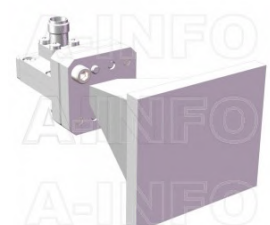
LB-180500-2.4FSPO Broadband Horn Antenna 18-50GHz 15dB Gain 2.4mm Female
