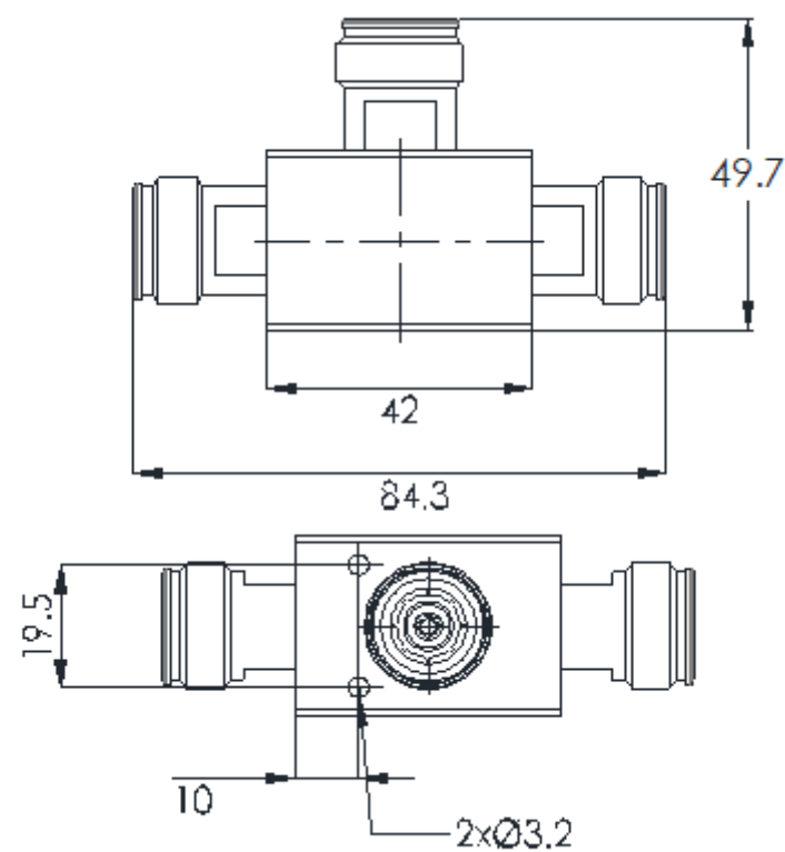
Product Drawing
