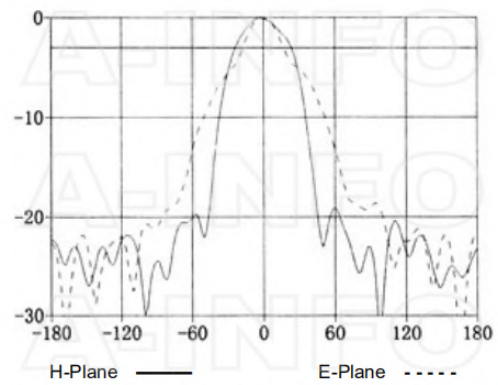
Frequency: 4.0GHz
