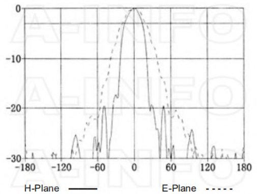
Frequency: 14.0GHz
