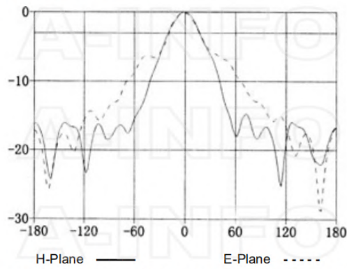
Frequency: 3.0GHz
