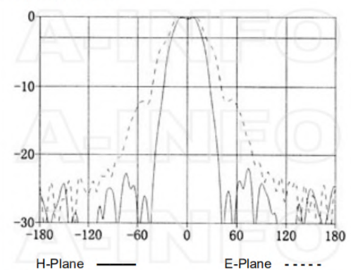
Frequency: 8.0GHz
