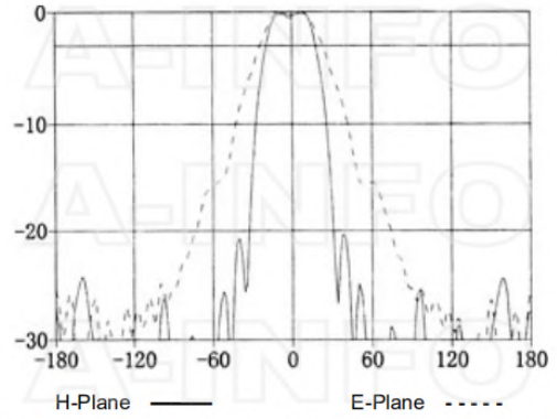
Frequency: 10.0GHz
