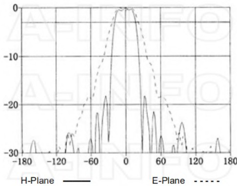
Frequency: 12.0GHz
