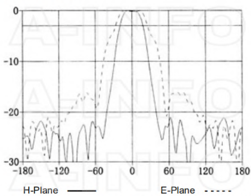
Frequency: 7.0GHz
