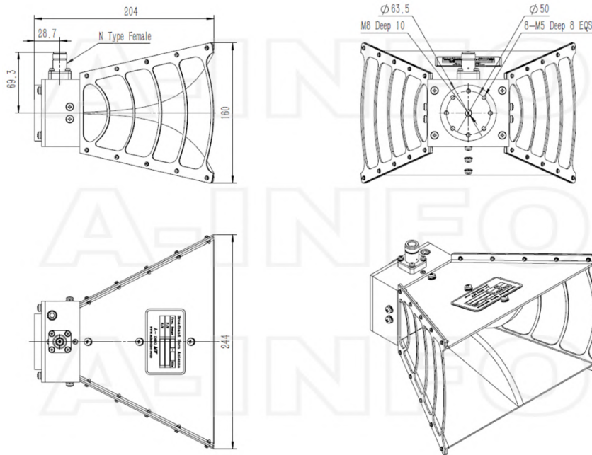
N-Female Output (P/N: LB-10200-NF)
