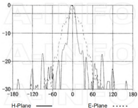
Frequency: 16.0GHz
