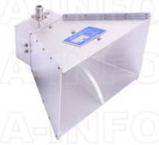
LB-10180-NFP Broadband Horn Antenna 1-18GHz 11dB Gain N Type Female
