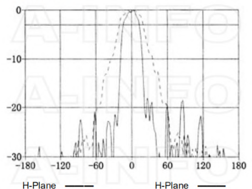
Frequency: 18.0GHz
