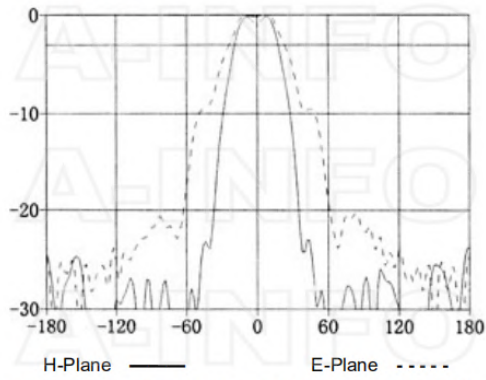
Frequency: 9.0GHz
