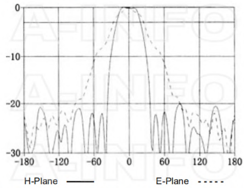
Frequency: 6.0GHz
