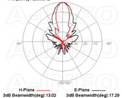
Frequency:12.00GHz
