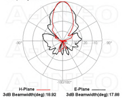
Frequency:7.00GHz
