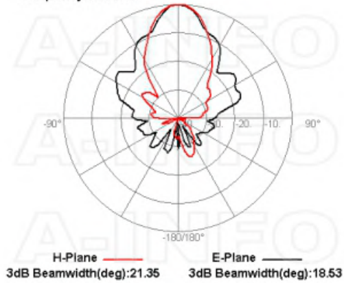
Frequency:6.00GHz
