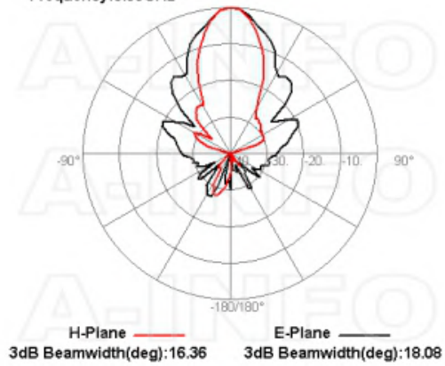
Frequency:8.00GHz
