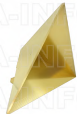
TCR-609.6 Radar Trihedral Corner Reflector 24inch(609.6mm) Edge Size
