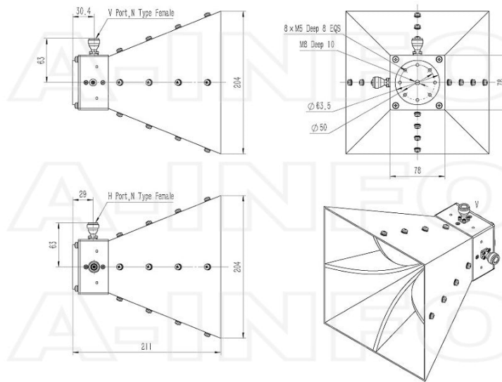
N-Female Output (P/N: LB-SJ-10100-NF)
