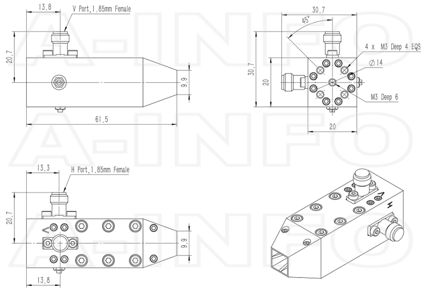
1.85mm-Female Output (P/N: LB-SJ-180670L-1.85F)
