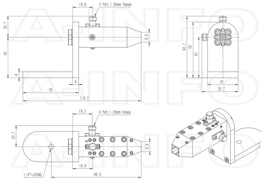
1.85mm-Female Output with L Type Mounting Bracket (Option, P/N: LB-SJ-180400-L)
