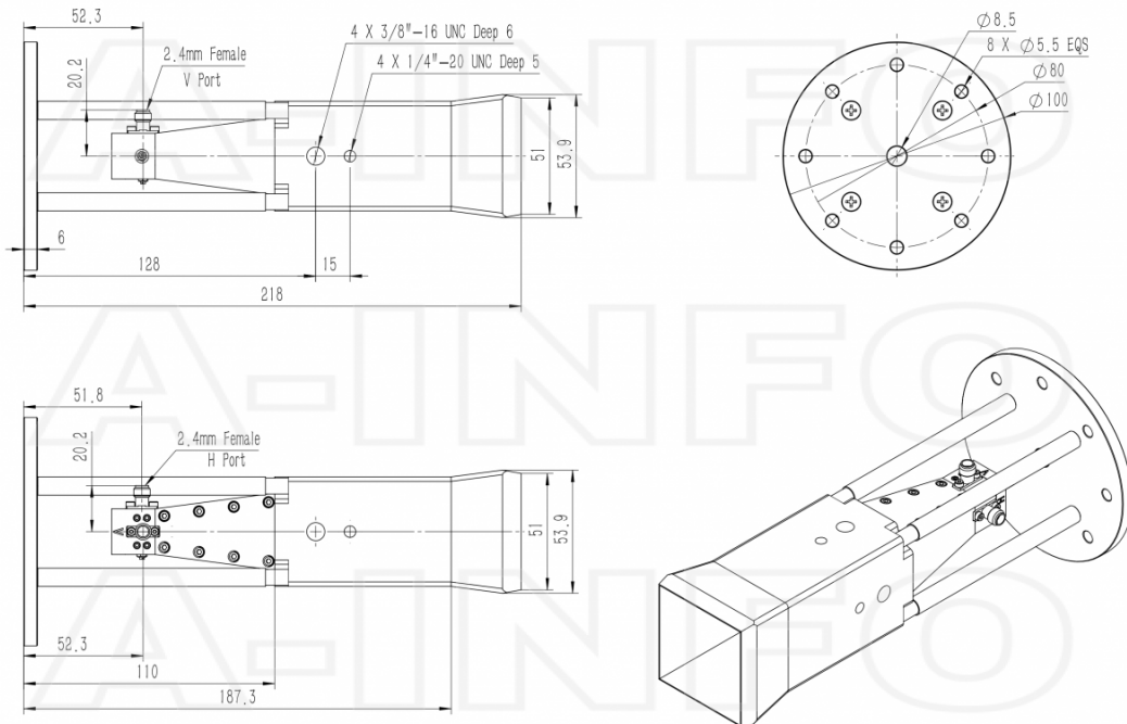
2.4mm-Female Output with Round Type Mounting Bracket (Option, P/N: LB-SJ-180500H-MB)
