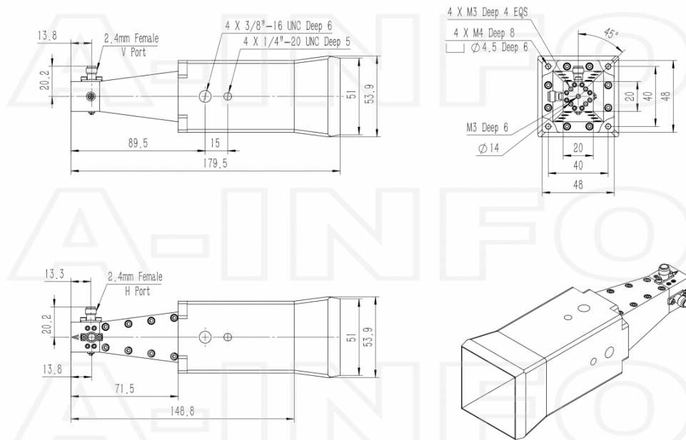
2.4mm-Female Output (P/N: LB-SJ-180500H-2.4F)
