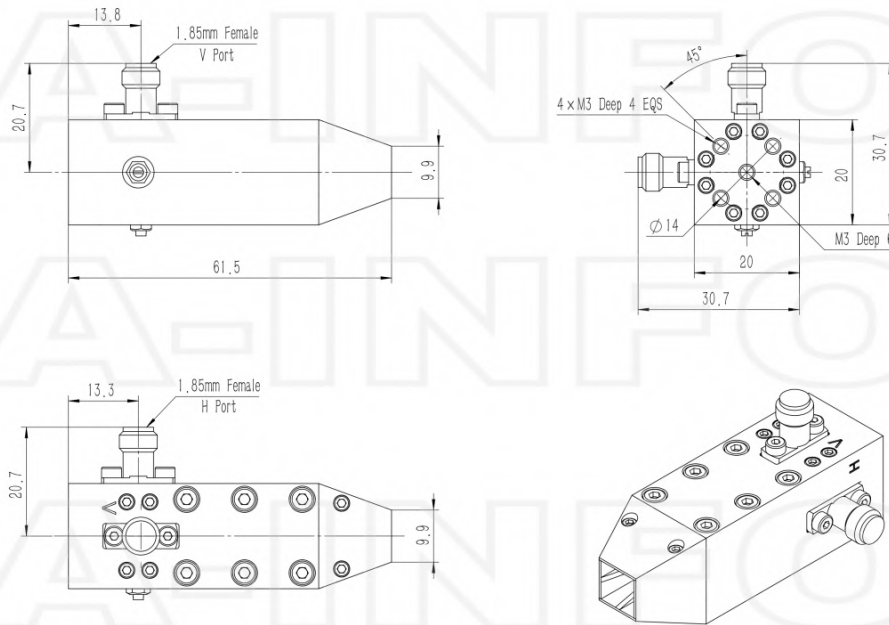
1.85mm-Female Output (P/N: LB-SJ-180500L-1.85F)
