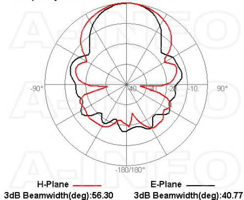
Frequency:5.000GHz
