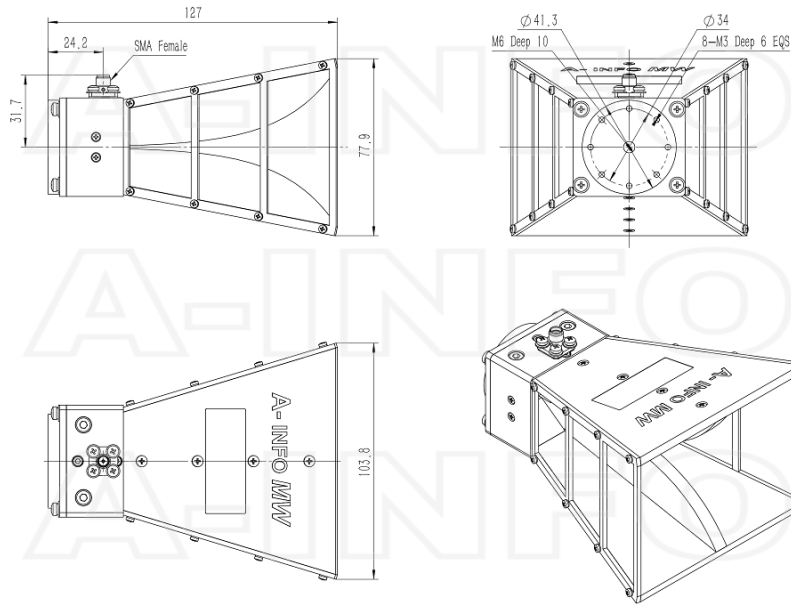
SMA-Female Output (P/N: LB-2020-SF)
