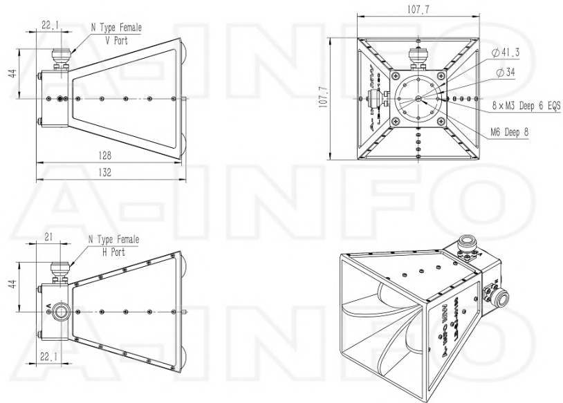
NFemale Output (P/N: LB-SJ-40180-NF)
