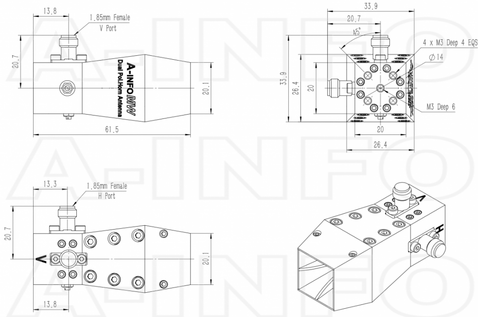
1.85mm-Female Output (P/N: LB-SJ-180540B-1.85F)
