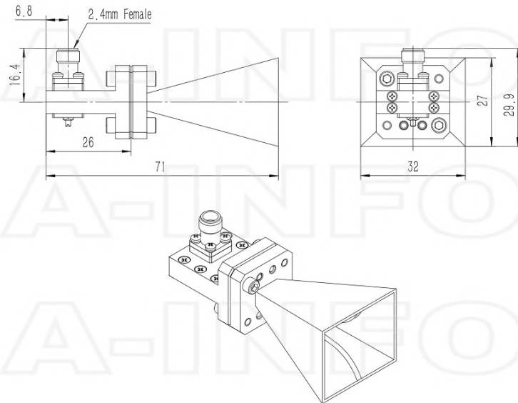
2.4mm-Female Output (P/N: LB-180400-2.4F)
