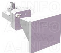
LB-180400-2.4FSPO Broadband Horn Antenna 18-40GHz 15dB Gain 2.4mm Female
