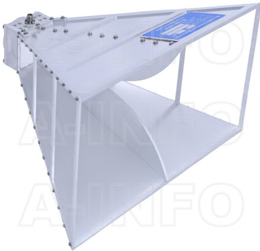
LB-8300-KF Broadband Horn Antenna 0.8-30GHz 12dB Gain 2.92mm Female
