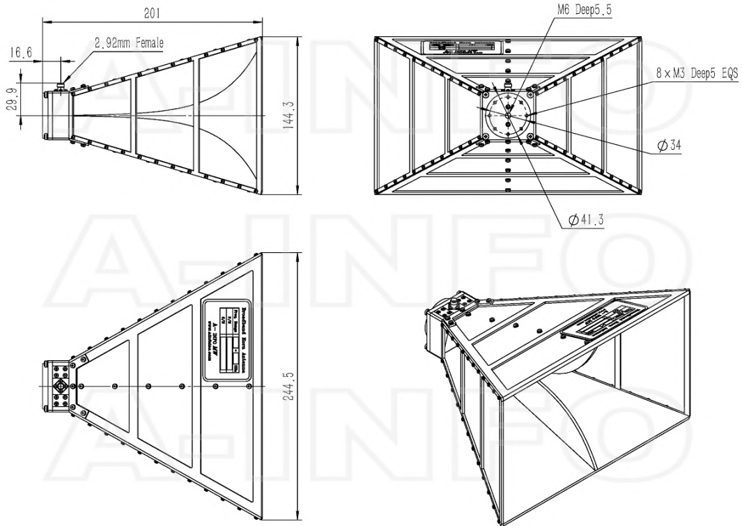
2.92mm-Female Output (P/N: LB-8300-KF)
