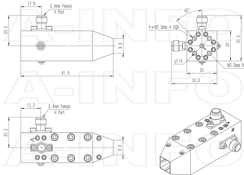
2.4mm-Female Output (P/N: LB-SJ-180400L-2.4F)
