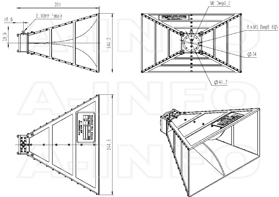
2.92mm-Female Output (P/N: LB-8400-KF)
