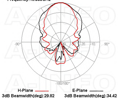
Frequency:18.000GHz
