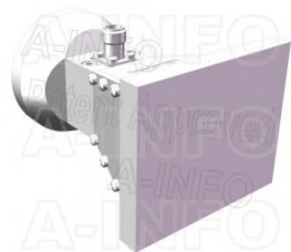
LB-45500-2.4FSPO Broadband Horn Antenna 4.5-50GHz 13dB Gain 2.4mm Female
