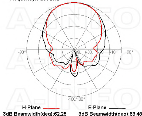
Frequency:7.000GHz
