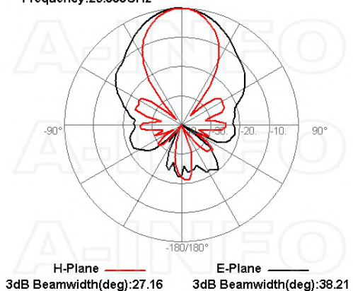
Frequency:26.000GHz
