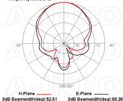
Frequency:6.000GHz
