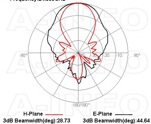
Frequency:24.000GHz
