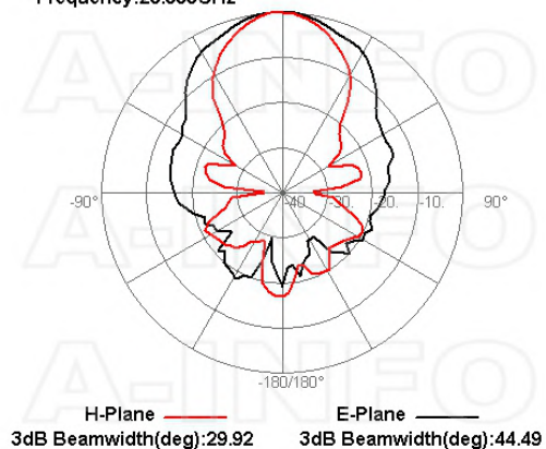
Frequency:20.000GHz
