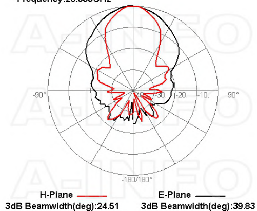
Frequency:28.000GHz
