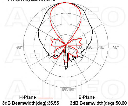
Frequency:22.000GHz
