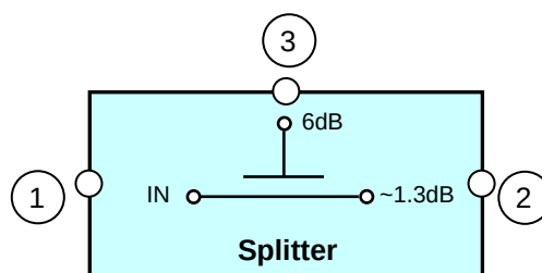
block diagram
