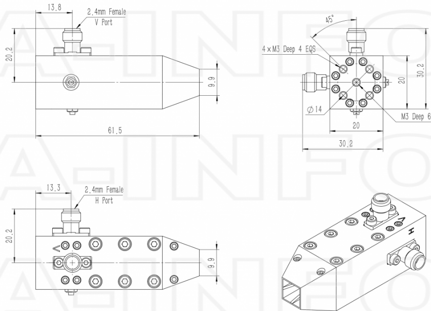
2.4mm-Female Output (P/N: LB-SJ-180500L-2.4F)
