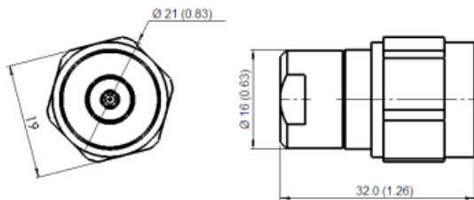
N-TER-01_02 sketch
